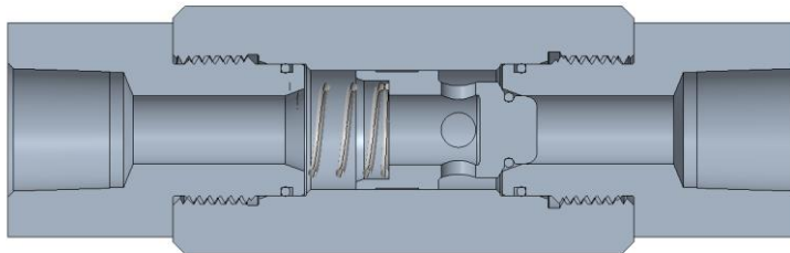
K3-101 : 3/4" NPT, 15,000 psi
