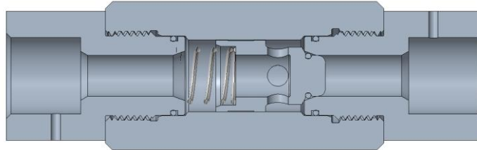
K3-100 : 3/4" MP 20,000 psi
