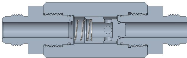
K3-102 : -12 JIC, 5,000 psi
